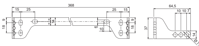
Staffa unica basculante / Single pivoting bracket
